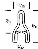
CMZ-9/16Y 9/16" Contoured Outer Bar
